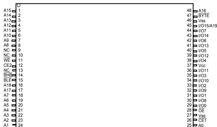
Figure 3. 48-pin TSOP I (512 K × 16/1 M × 8) (Top View) [1, 3]
